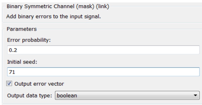
Рис. 3.48. Binary Symmetric Channel
